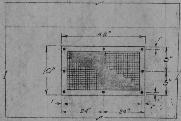
CIRCUMFERENTIAL VENT SCREEN DETAIL
